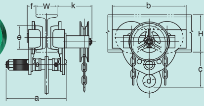
AGD Geared Trolley (Drop Stop)
