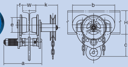
AG Geared Trolley
