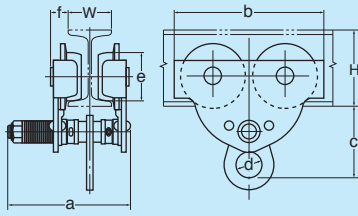
APD Plain Trolley (Drop Stop)
